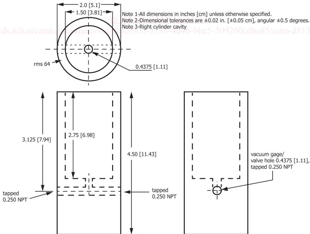
FIG. 1 Apparatus Design
