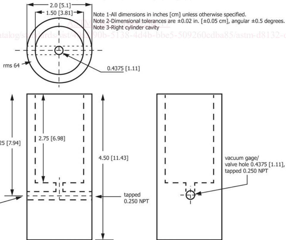
FIG. 1 Apparatus Design
