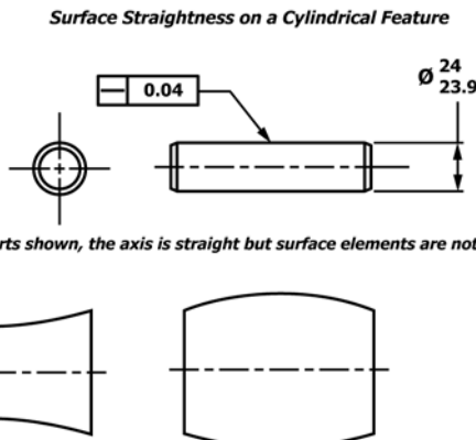
FIG. 1 Definition of a “Straight” Condition
