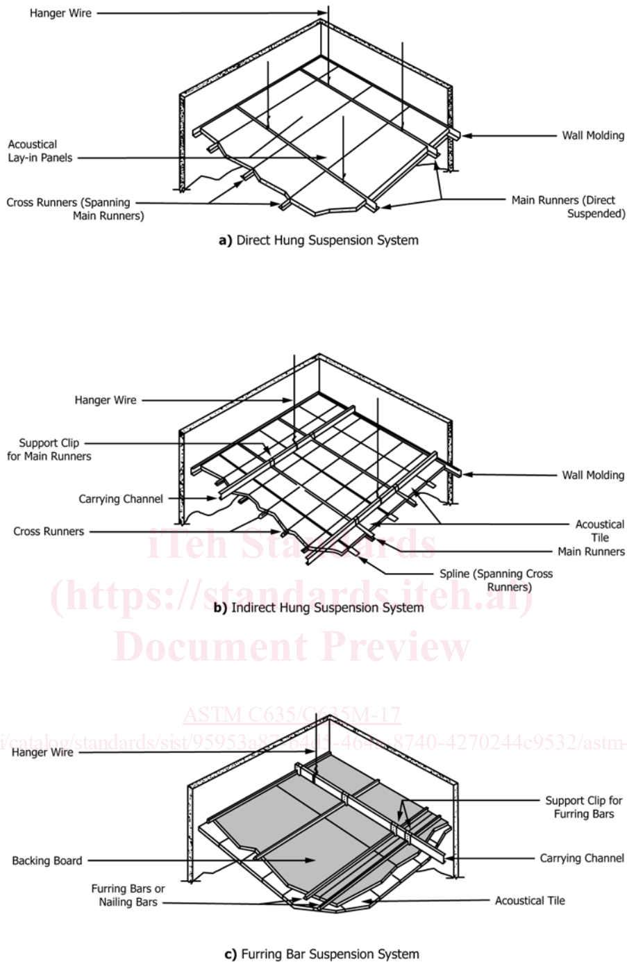
FIG. 1 Three Types of Ceiling Suspension Systems Showing All Components
