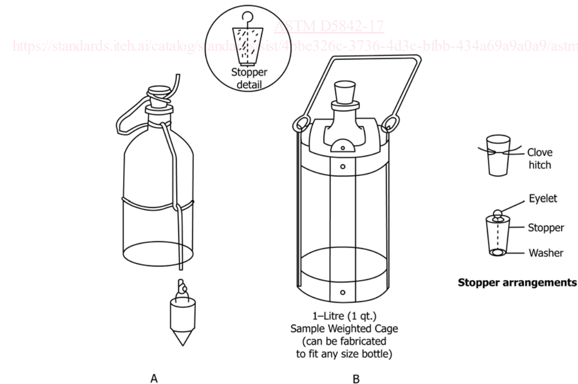
FIG. 3 Assembly for Bottle Sampling
