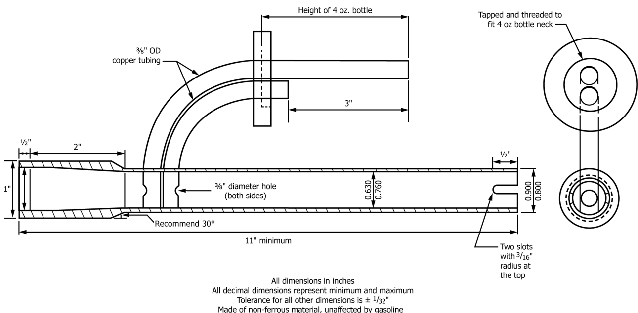
FIG. 1 Nozzle Extension for Nozzle Sampling with 4-oz-4 oz Bottle
