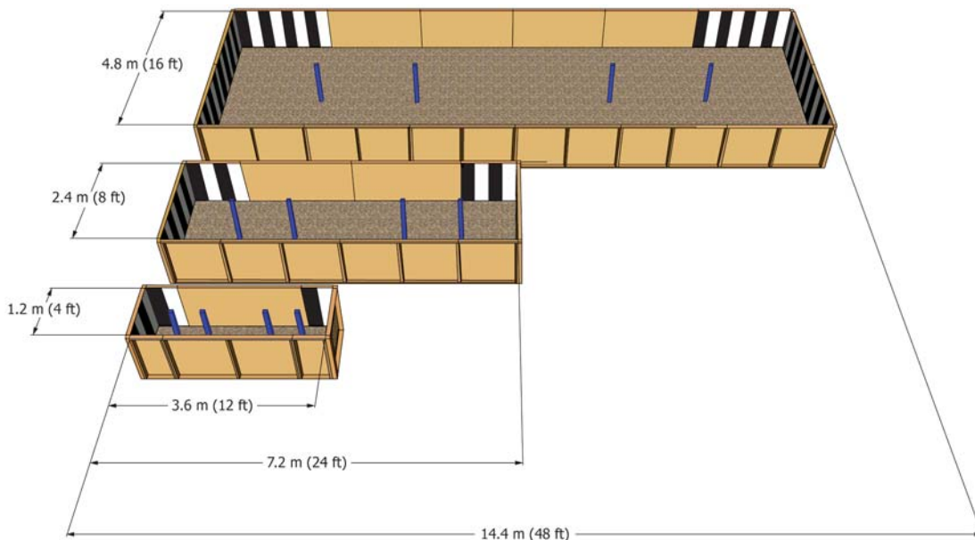
FIG. 1 Confined Area Terrains: Sand; Three Sizes
