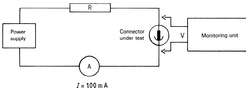
Figure 2 — Resistance monitor
