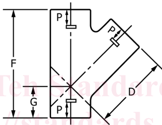
FIG. 8 Long-Sweep Quarter Bends
