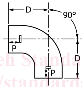
FIG. 1 No-Hub Pipe (MJ)
