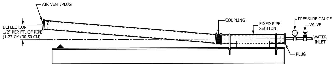
FIG. 5 Deflection Test
