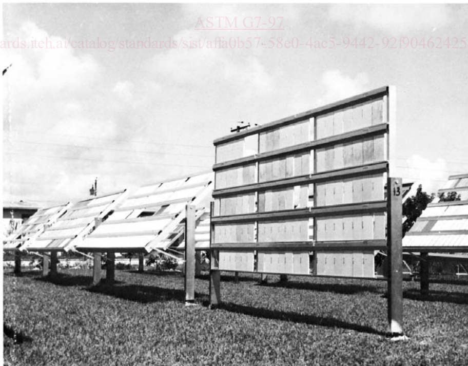
NOTE 1—Detailed drawings of this test rack may be obtained from ASTM Headquarters, 100 Barr Harbor Dr., W. Conshohocken, PA 19428. Request Adjunct No. 12-700070-00.
