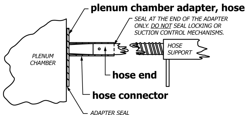
FIG. 21 Diagram of Hose and Adapter Connection
