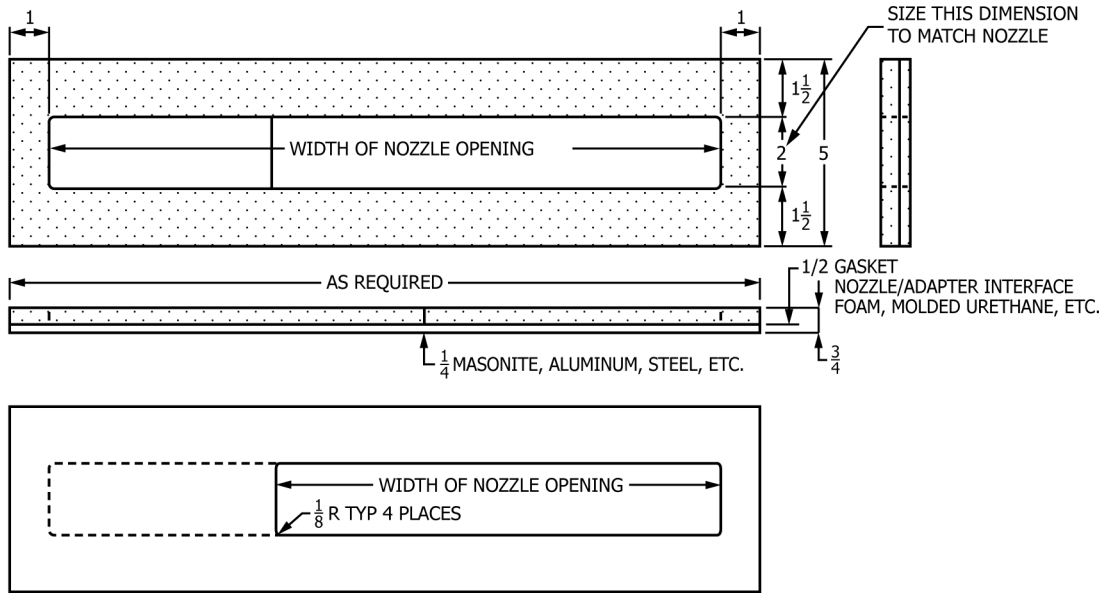
FIG. 43 Nozzle Adapter
