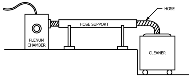
FIG. 32 Schematic for Air Performance Test
