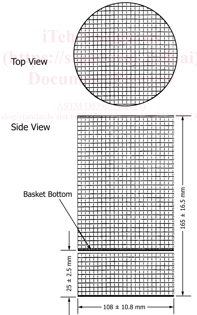
FIG. 1 Wire Basket Assembly (Not to Scale)
