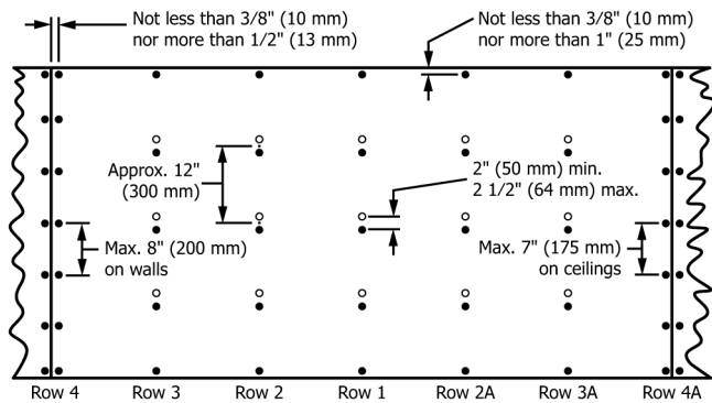
FIG. 3 Double Nailing
