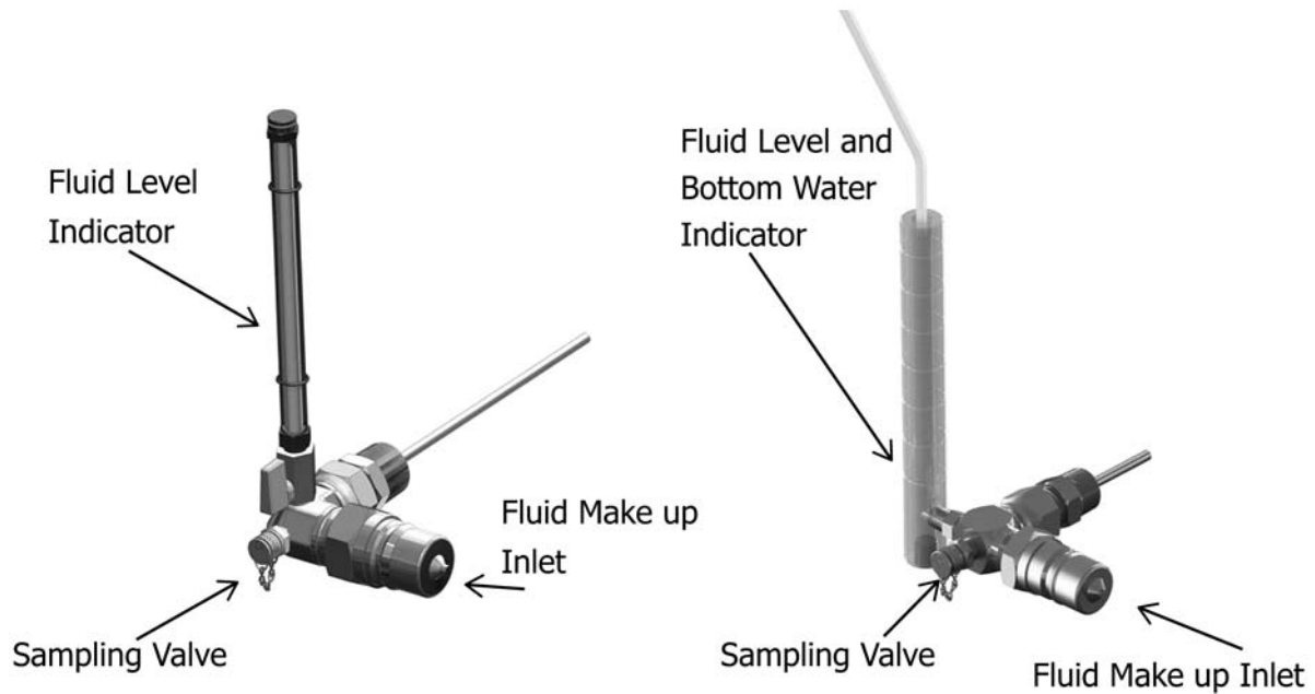
FIG. 8 Common Arrangements of Sampling Valve, Fluid Level Indicator and Fluid Make-up Inlet
