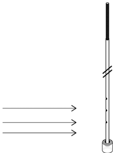
FIG. 4 Example of a Weighted Drop Tube Device
