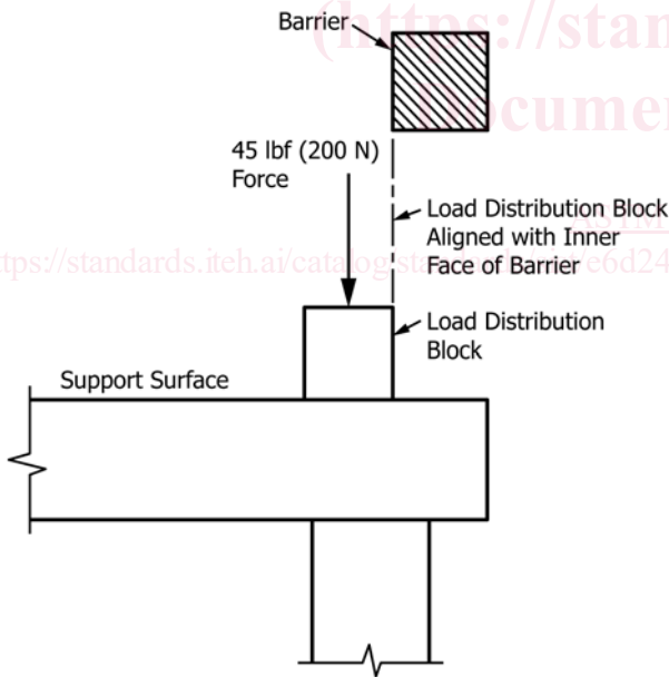
FIG. 4 Stability Test
