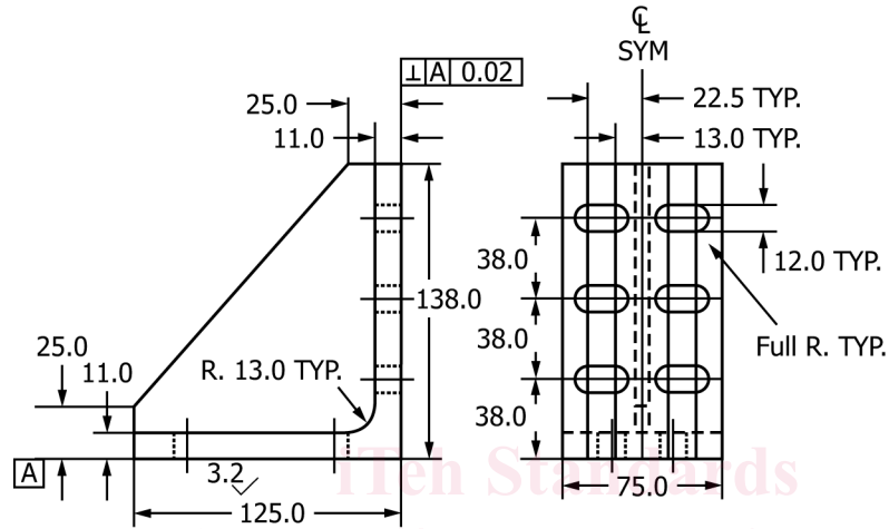
FIG. 6 Support Fixture Angles (SI Version)
