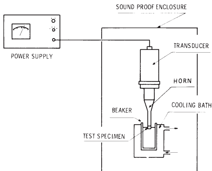
FIG. 2 Schematic of Vibratory Cavitation Erosion Apparatus
