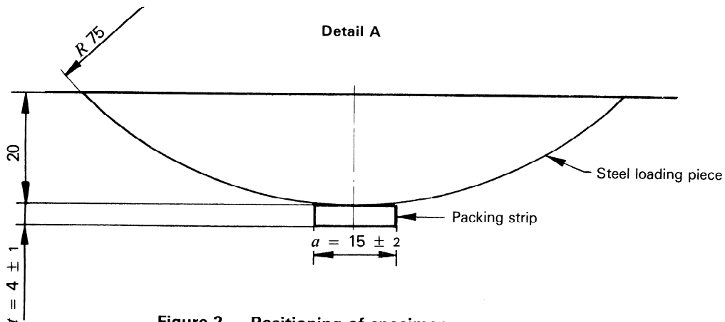
Figure 2 – Positioning of specimen
