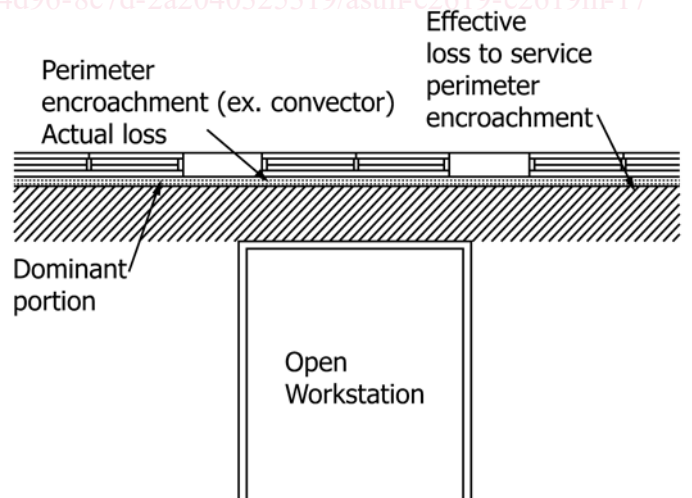
FIG. 9 Actual and Effective Losses Due to Restricted Area Kept Clear to Permit Service of Encroachment (Convactor)
