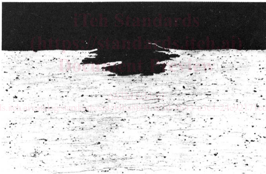
Undermining pitting that may form the surface give the appearance of incipient exfoliation (Keller's Etch; 100×).
