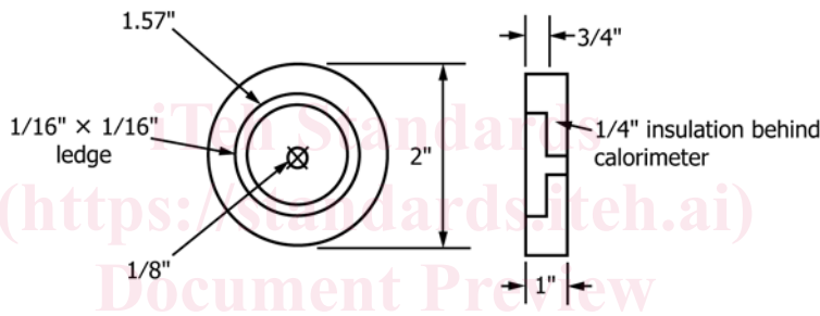
FIG. 5 Sensor Mount
