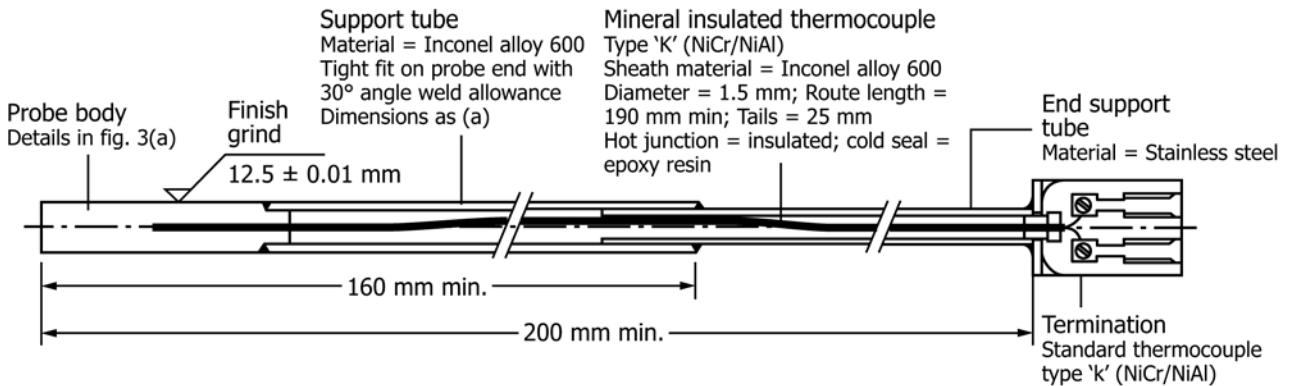
FIG. 2 Probe Details and General Probe Assembly
