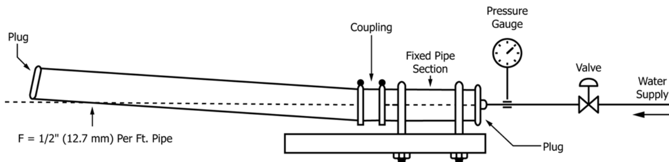
FIG. 1 Deflection Test
