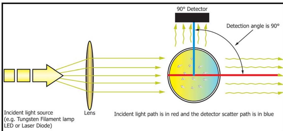
FIG. 1 Photoelectric Nephelometer
