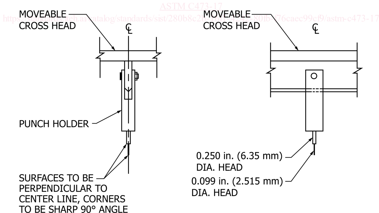
FIG. 5 Test Setup—Punch for Hardness and Nail Pull Resistance
