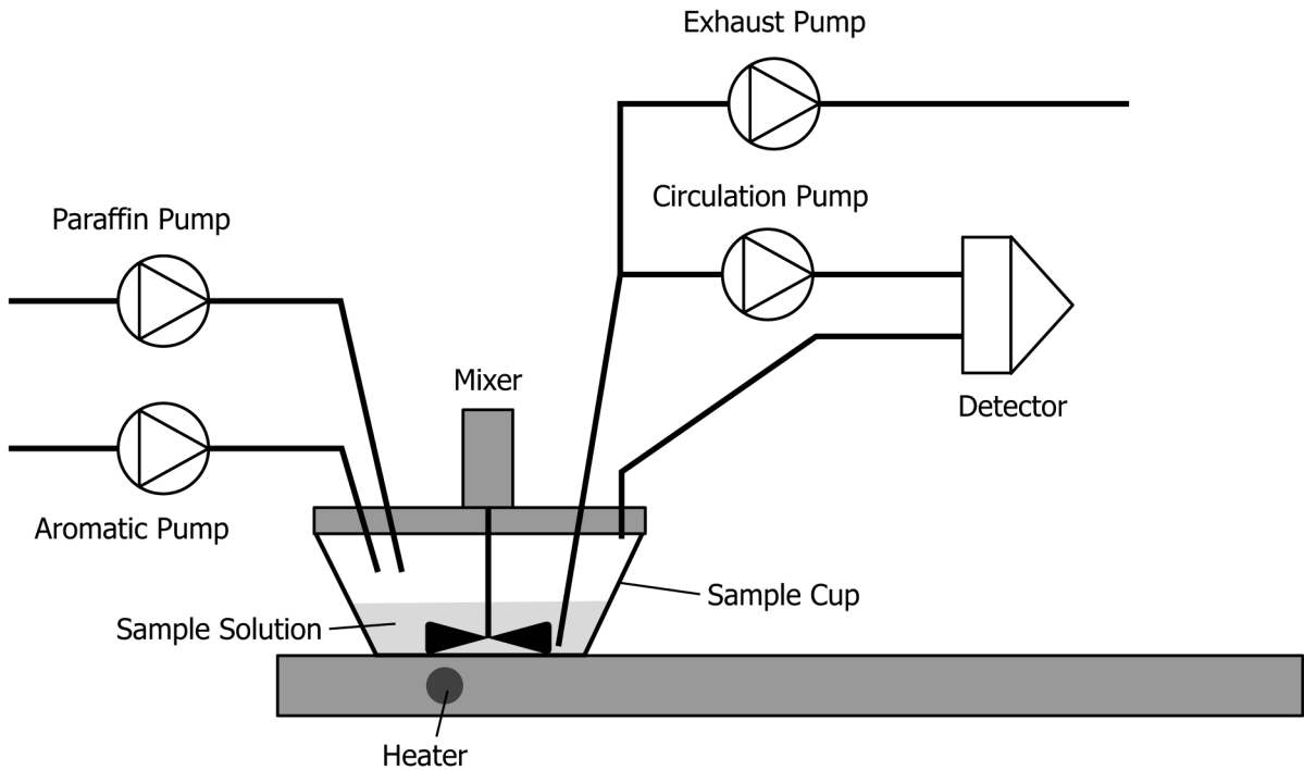
FIG. 2 Schematic Diagram of PORLA Heavy and Crude Oil Stability and Compatibility Analyzer
