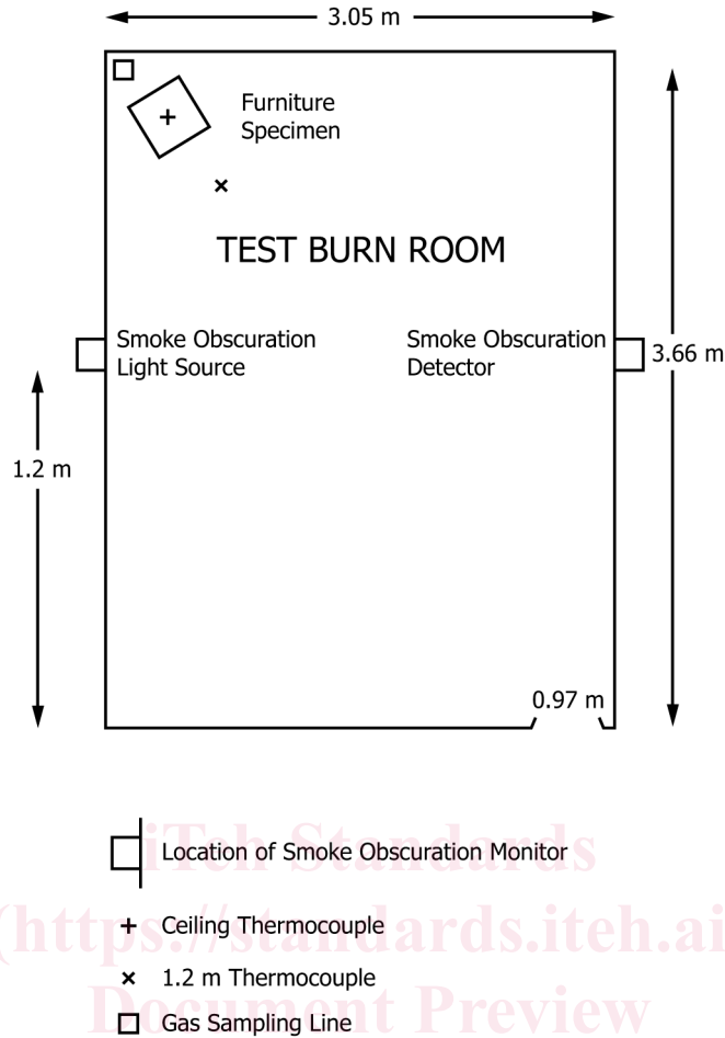
FIG. 2 Test Room Configuration for Test Configuration B
