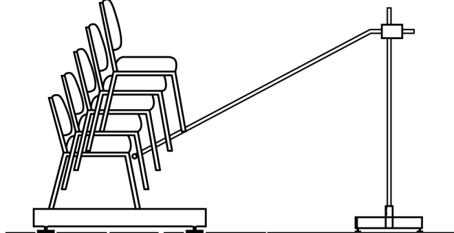
FIG. 4 Positioning of the Ignition Source—T Burner
