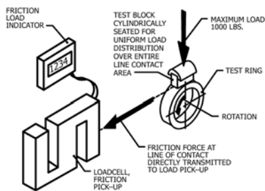
FIG. 1 Test Schematic
