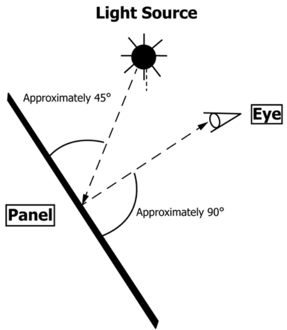
FIG. 1 Test Panel
