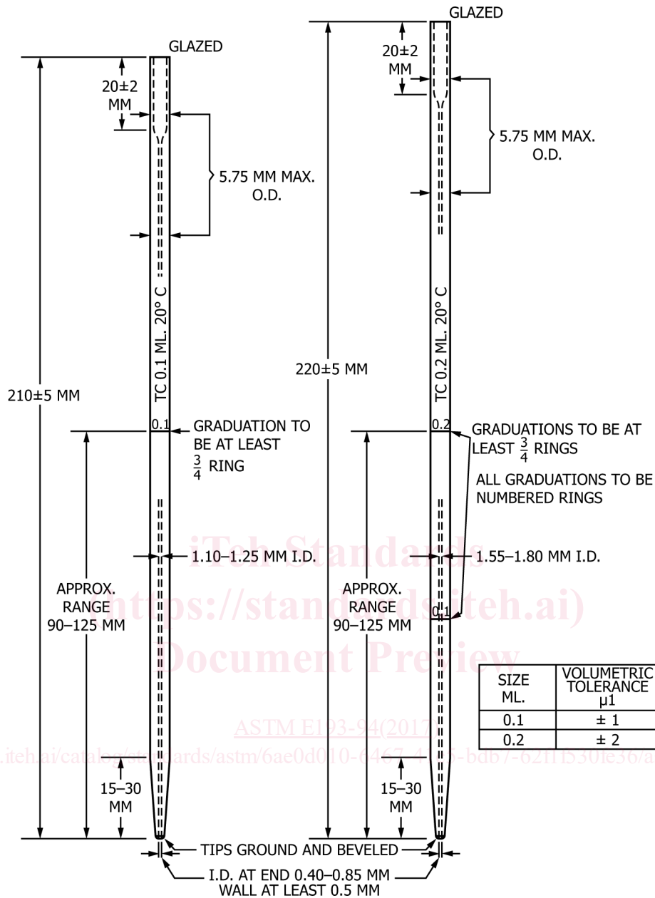
FIG. 2 Micropipets, Folin-Type
