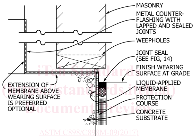
FIG. 4 Terminal Condition with Masonry Above Finish Wearing Surface at Grade (see 7.6.1) c898m-092017
