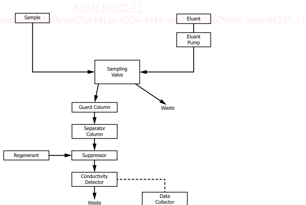
FIG. 2 Schematic of an Ion Chromatograph
