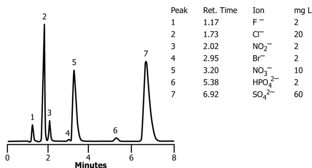
FIG. 1 Chromatogram Showing Separation Using the AS4A Column
