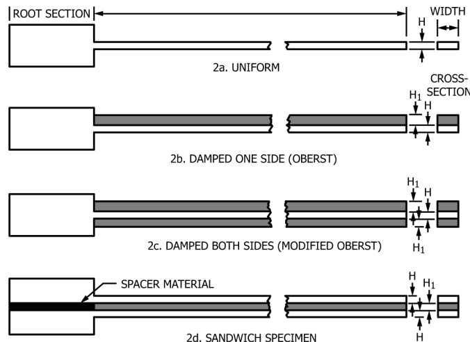
FIG. 2 Test Specimens
