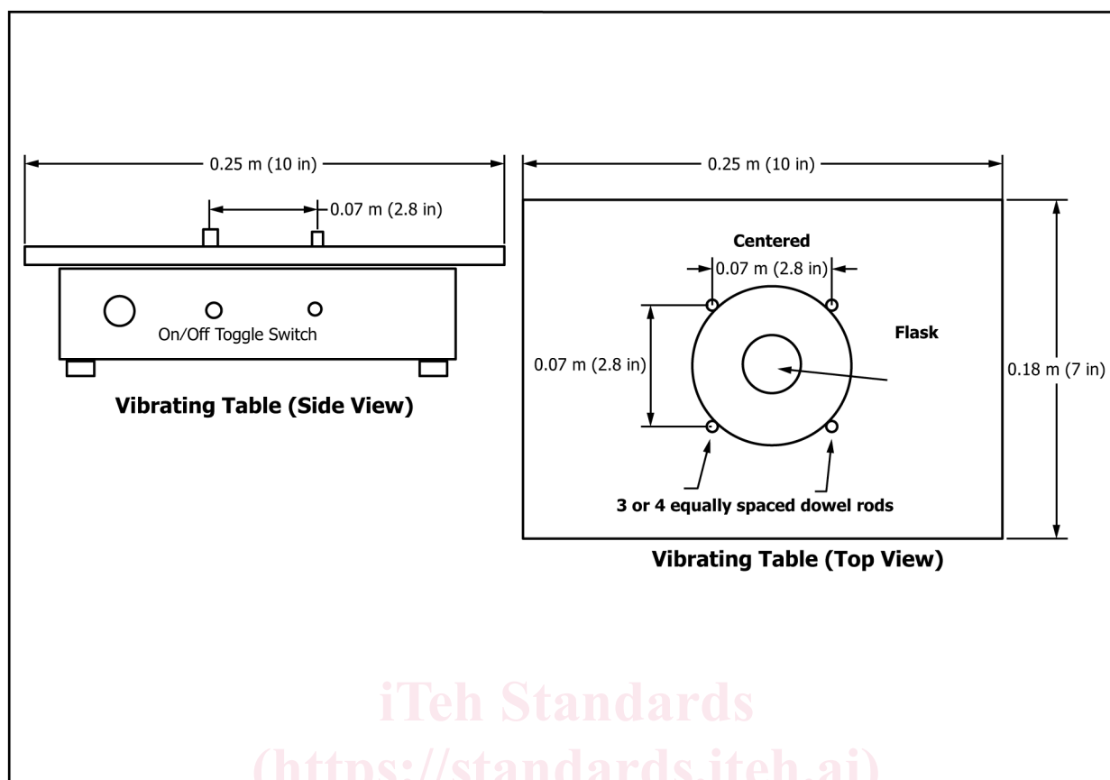
FIG. 1 Vibrating Table
