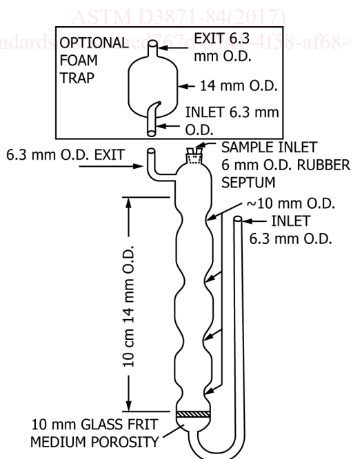
FIG. A1.1 Purging Device
