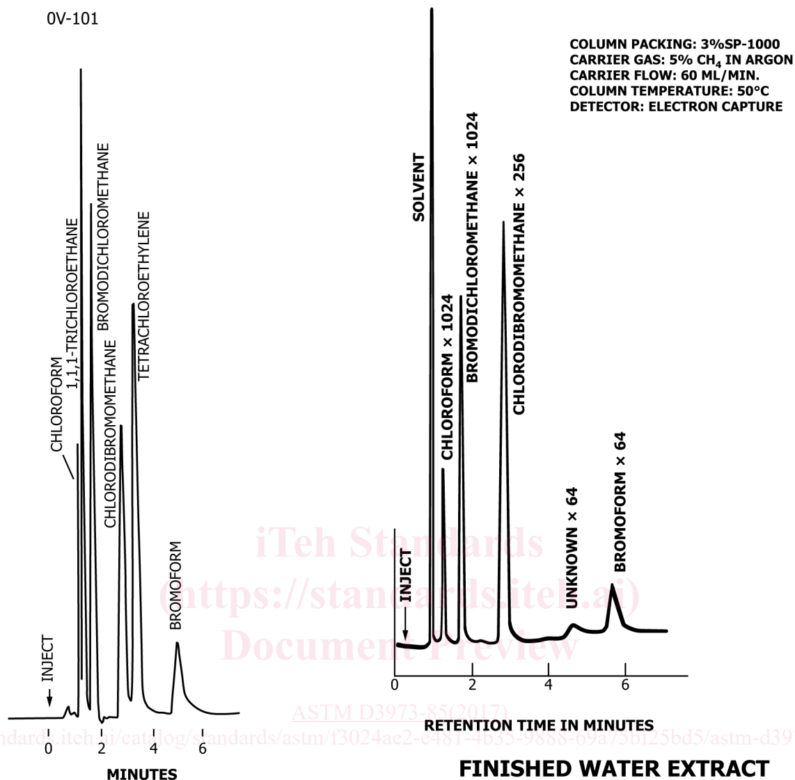
FIG. 1 Chromatograms of Standards
