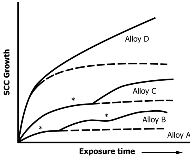
FIG. 1 Effect of Corrosion Product Wedging on Growth Crack Versus Time Curve
