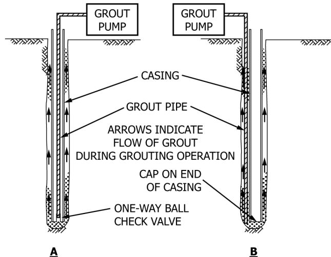
CROSS-SECTION VIEW
