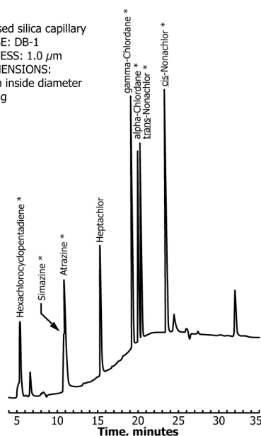
FIG. 2 Extract of Reagent Water Spiked at 20 µg/L with Atrazine, 60 µg/L with Simazine, 0.45 µg/L with Cis-nonachlor, and 0.35 µg/L with Hexachlorocyclopentadiene, Heptachlor, Alpha Chlordane, Gamma Chlordane, and Trans-nonachlor
