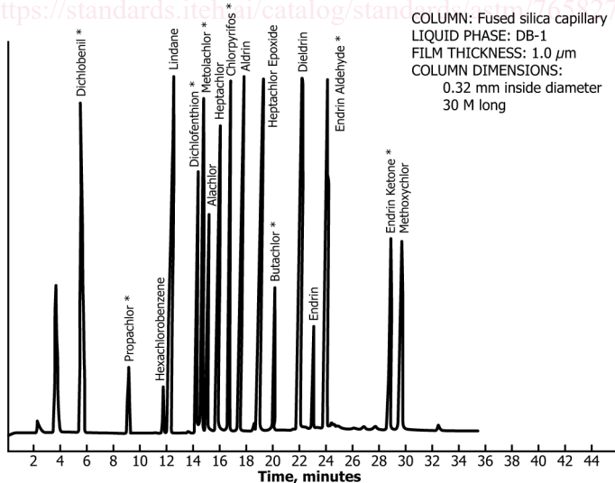
FIG. 1 Hexane Spiked at 7.71 µg/L with Heptachlor and Lindane; 9.14 µg/L with Heptachlor Epoxide; 11.4 µg/L with Aldrin and Hexachlorobenzene; 23 µg/L with Butachlor, Chlorpyrifos, Chlorpyrifosmethyl, Dicllobenil, Dieldrin, Endrin, Metolachlor, and Propachlor; and 44.9 µg/L with Methoxychlor
