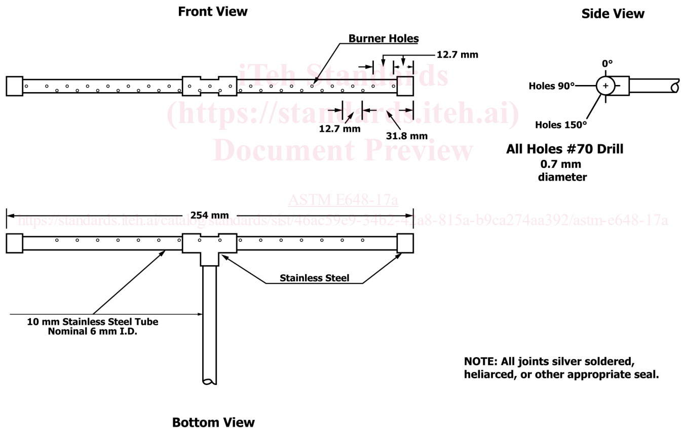
FIG. 6 Pilot Burner
