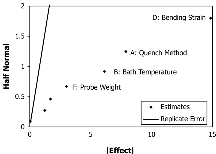
FIG. 1 Half-Normal Plot, Test Method F2082 Example
