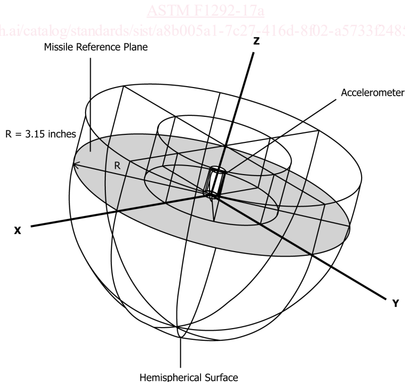
FIG. 1 Missile Reference Plane and Axes
