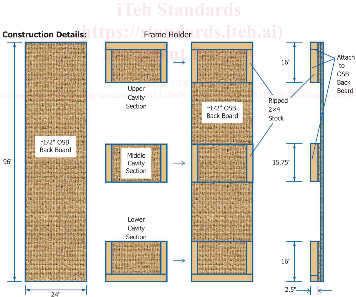
FIG. 1 Recommended Frame Holder (an Example)
