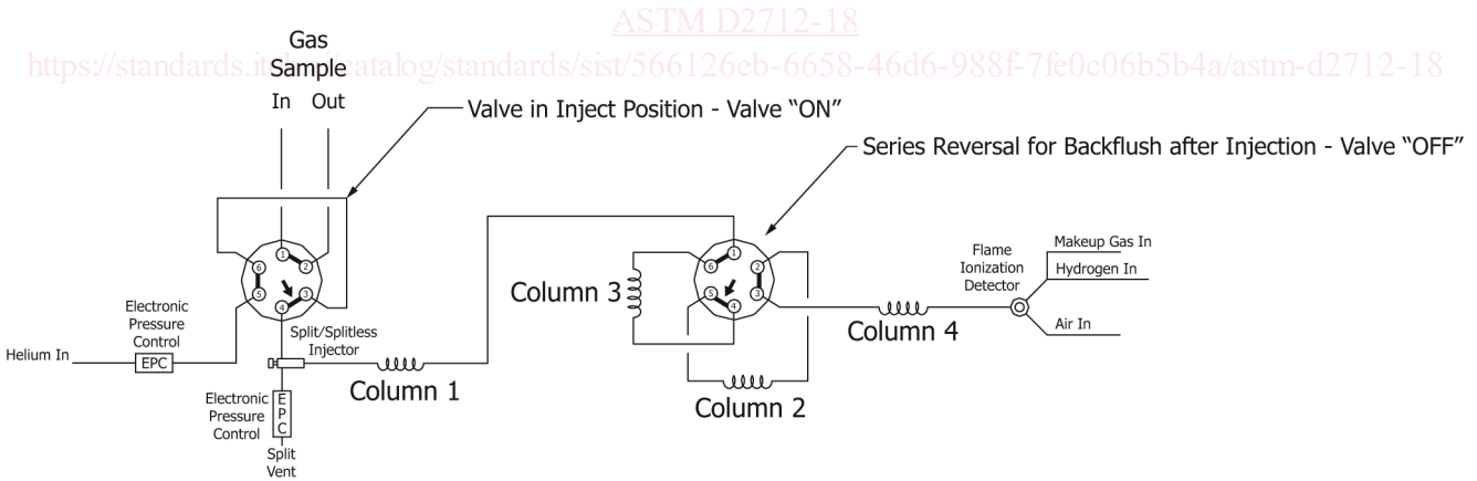
FIG. 4 Arrangement of Valves (Gas Sampling Valve Included)
