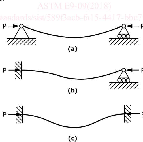
FIG. 1 Diagrams Showing Fixity Conditions and Resulting Buckling of Deformation
