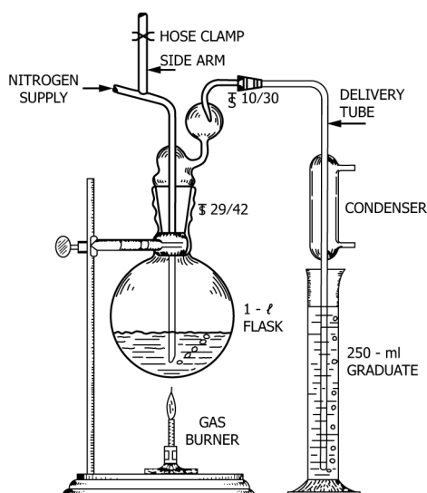
FIG. 3 Apparatus for Distillation of Chlorine
