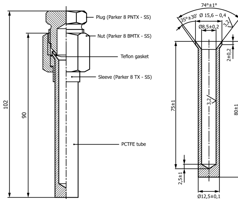
FIG. 1 Example of a Polychlorotrifluoroethylene P-10 Tube
