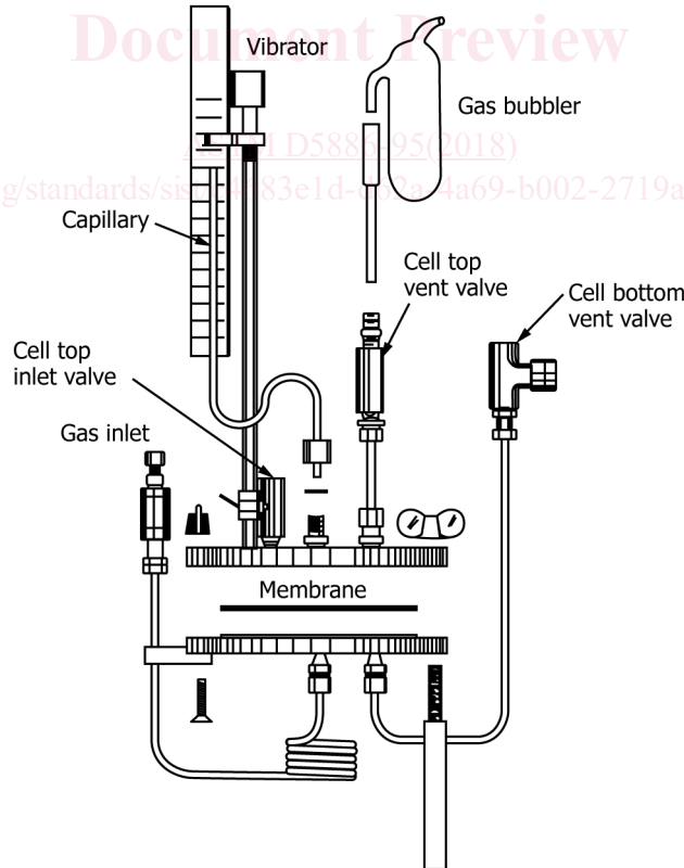
FIG. 1 Gas Permeability Apparatus in Test Method D1434, Procedure V—Volumetric—V – Volumetric (1)
