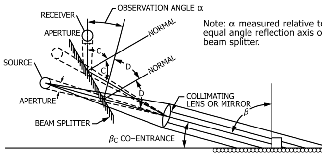
FIG. 2c Angles and apertures for portable retroreflectometer with collimating and beam splitter design
