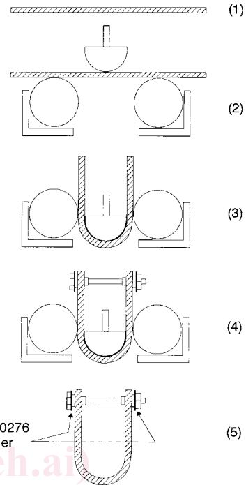
FIG. A1.2 Suggested Stressing Fixture (fastener inserted while specimen in die)
